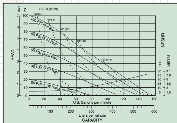
T20 Performance Curve
