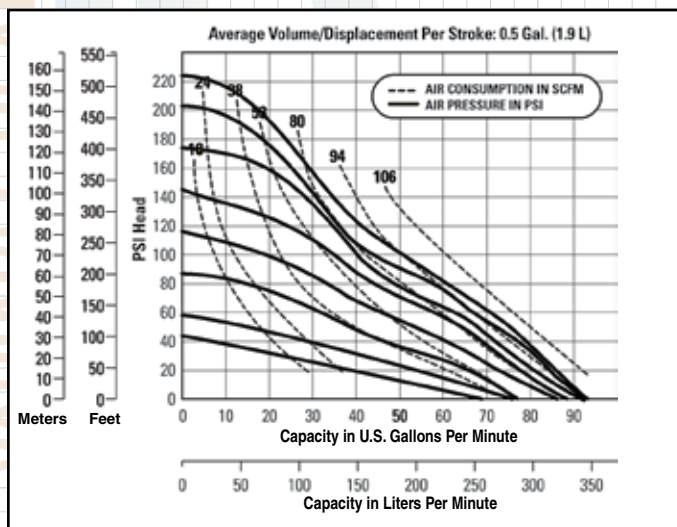
N50 Performance Curve
