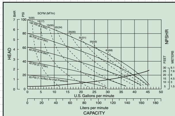
T1F Performance Curve
