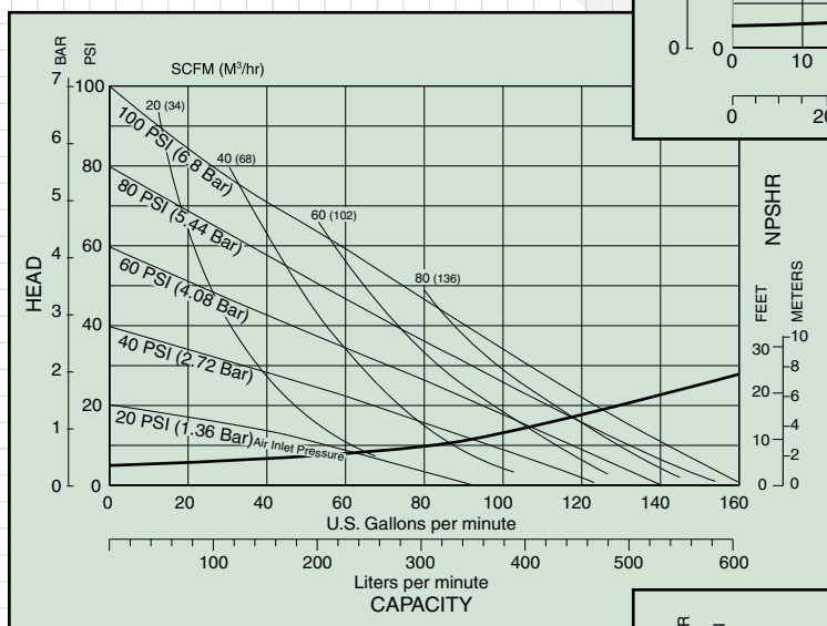
S20 Non-Metallic Performance Curve
