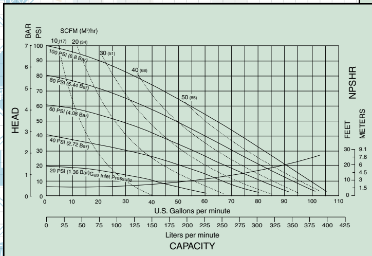
G20 Performance Curve
