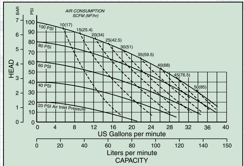
ST1-A Metallic Performance Curve
