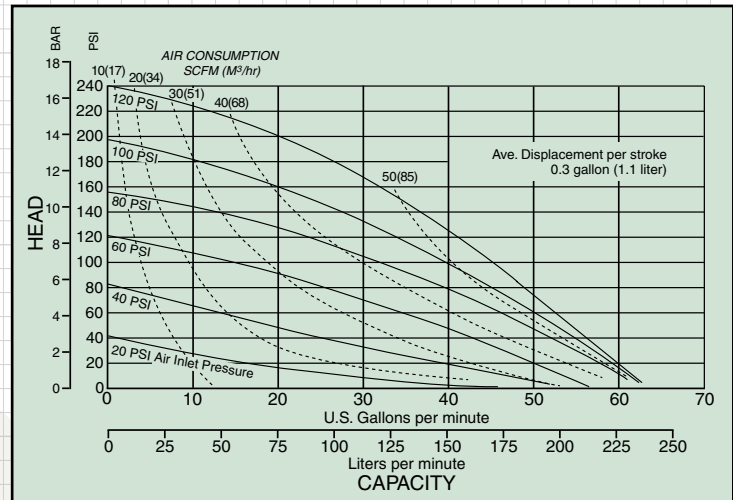
GH2-M Performance Curve
