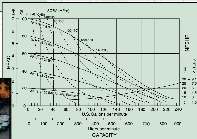
S30 Non-Metallic Performance Curve
